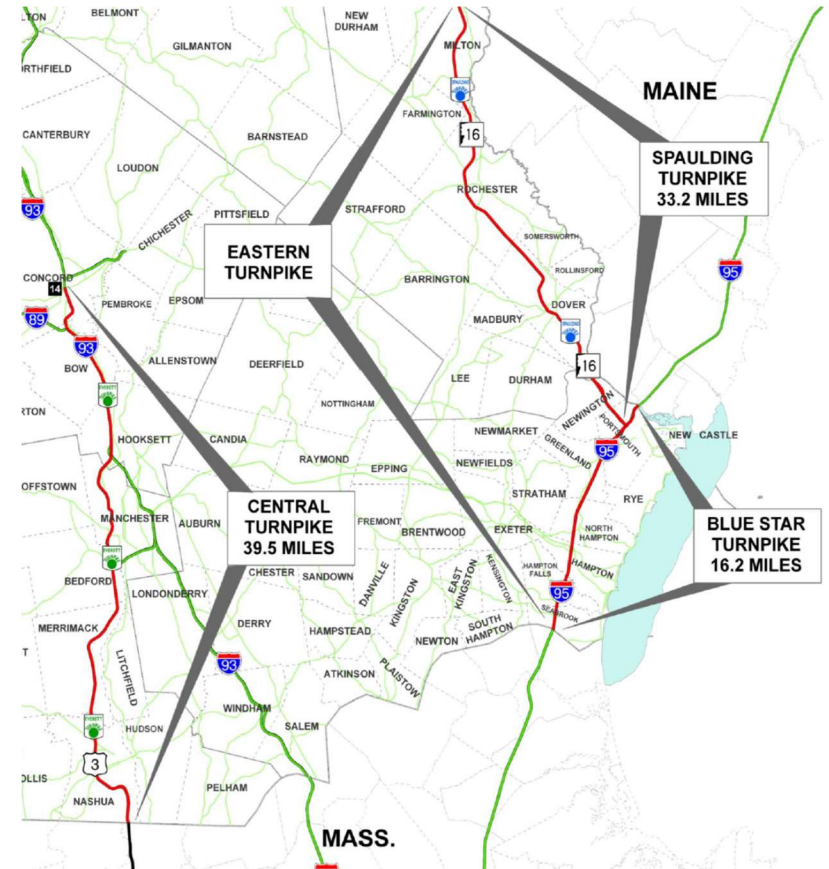
Turnpike System
