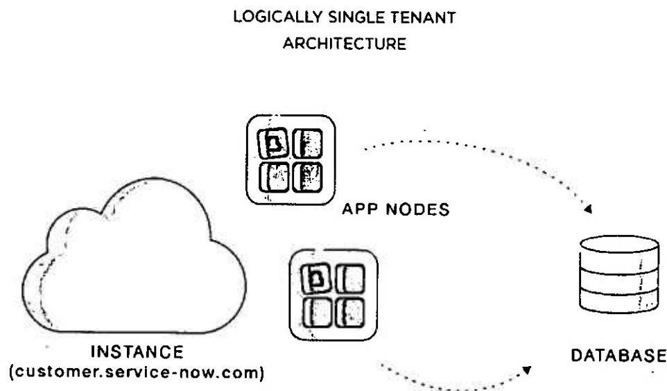
Figure 23: ServiceNow Architecture
