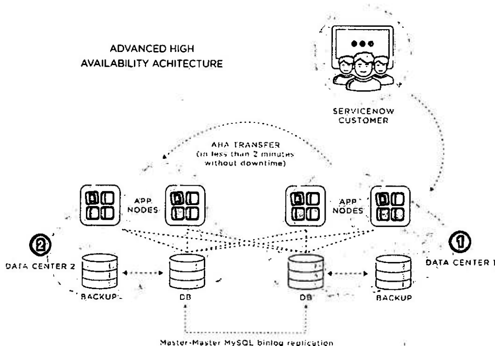
Figure 9: ServiceNow Architecture
